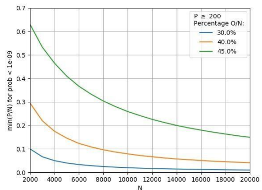
(b) P_{51} < 10^{-9}
