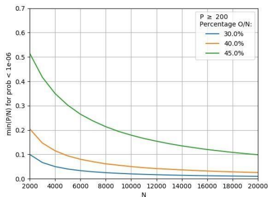
(a) P_{51} < 10^{-6}
